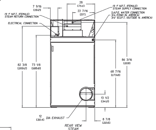
REAR VIEW STEAM
